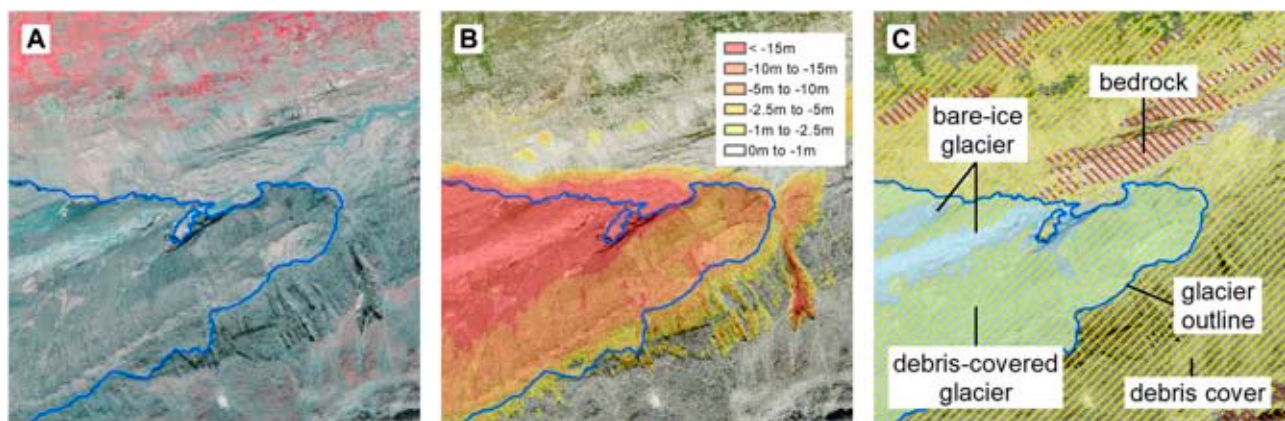
FIGURE 3 | The highly debris-covered tongue of Unteraargletscher in the Bernese Oberland as seen on the digital aerial images and used for mapping in 3D-views by swisstopo topographers. The combination of (A) infrared and (B) true color (RGB) combined with swissALTI 3D elevation differences (yellow to red colors) results in (C) swissTLM 3D object classes. The blue line in all panels indicates the swissTLM 3D object class “glacier.”
