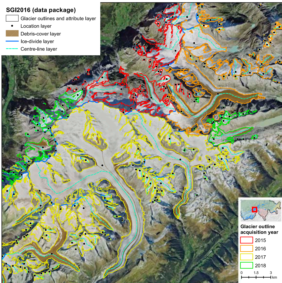
FIGURE 5 | Overview on the files provided with the SGI2016 data package in the area of Grosser Aletschgletscher. The glacier outlines are colored according to the acquisition year of the aerial image used for digitizing. Background: SWISSIMAGE orthoimagery composite.
