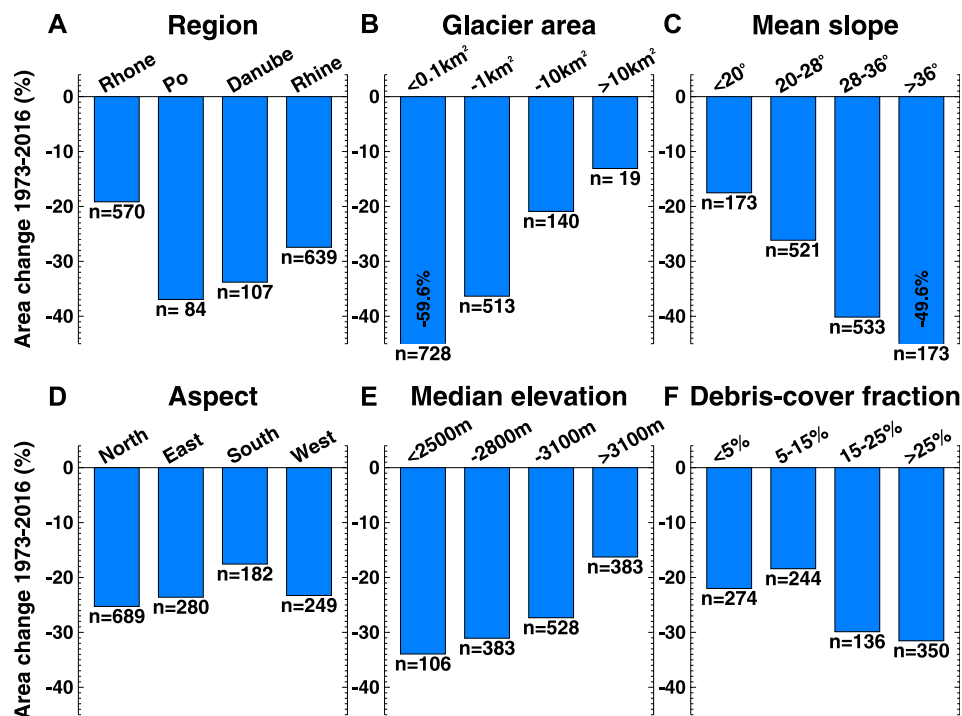
FIGURE 10 | Arithmetic mean of glacier-specific relative area changes 1973–2016 according to (A) the major catchment, and classes of (B) glacier area, (C) mean surface slope, (D) principal surface aspect, (E) median elevation, and (F) debris-cover fraction according to the SGI2016. The number of glaciers per class ( n ) is given.
