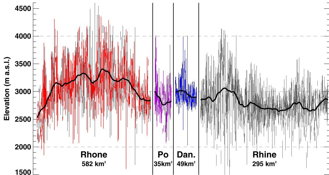
FIGURE 6 | Elevation range of all glaciers in the SGI2016, plotted per major river catchment, ordered from west to east (red, B: Rhone; purple, C: Po; blue E: Danube; grey, A: Rhine). Every colored line indicates the elevation range of a single glacier. The bold black line shows a running mean of the median.
